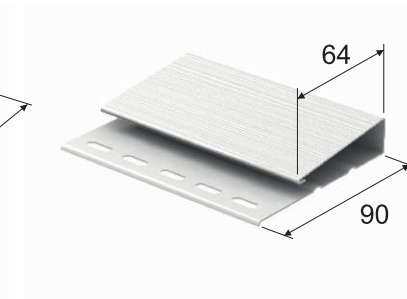
super J-trim
