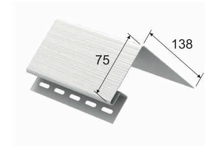
window flashing
