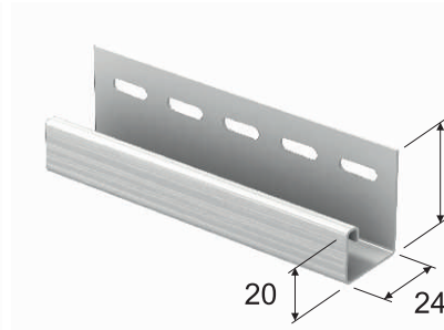
J-trim
